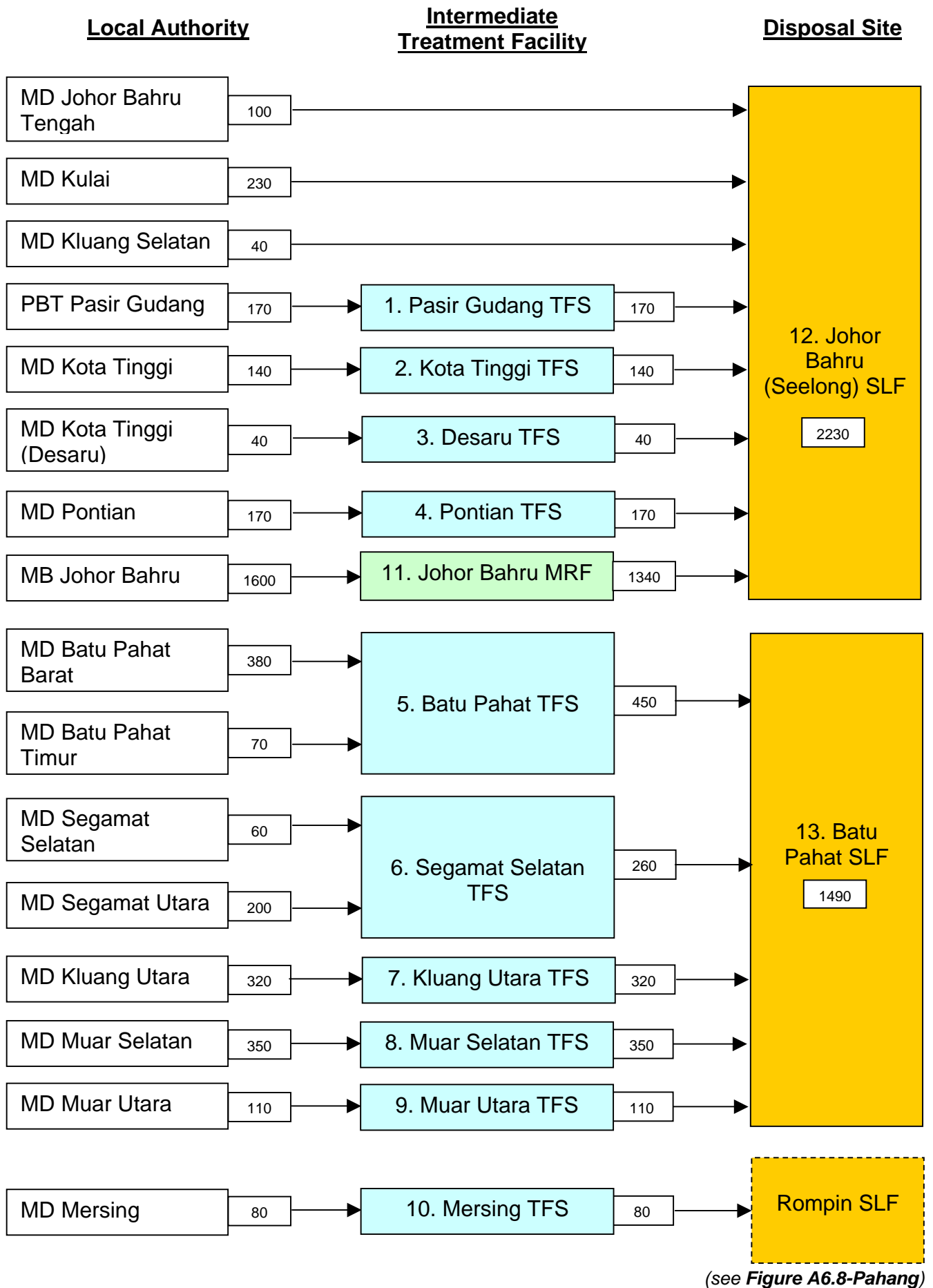
Figure 4.11 Waste Flow and SWM Facilities in Johor in 2020 (see Figure A6.8-Pahang)
